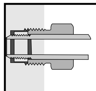
"M" Series Connection
