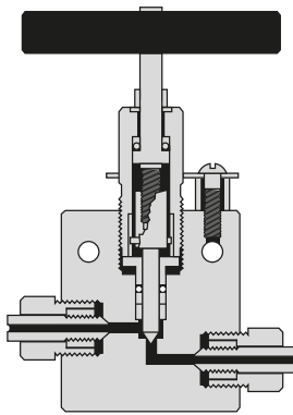
Positive Guide Stem
