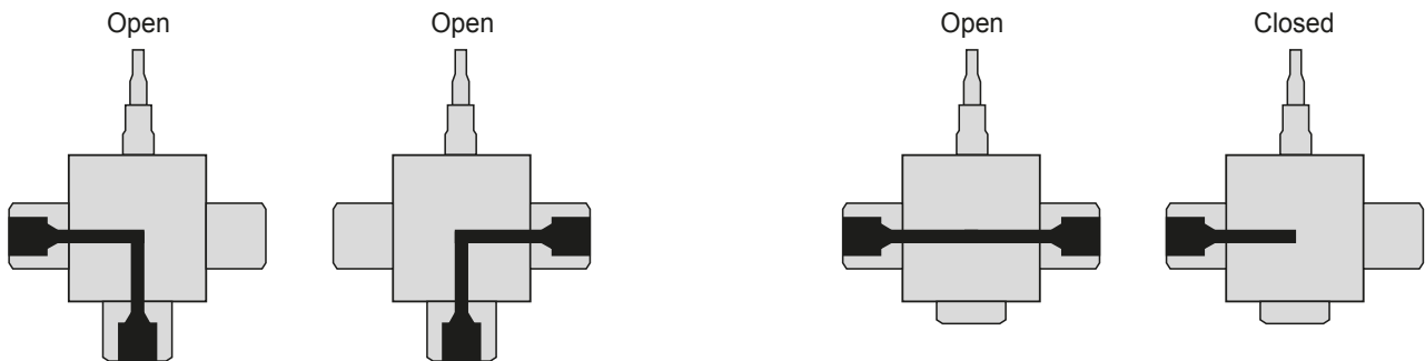
90° Three-Way Diverter Valve
