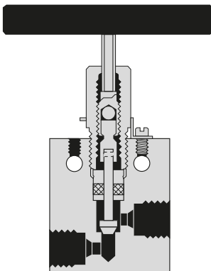
Pinned Stem
