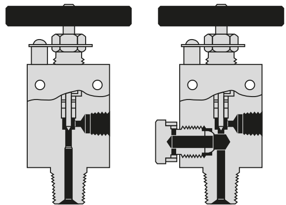
Without Safety Head
