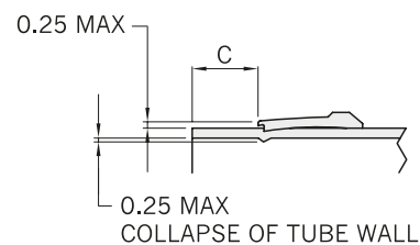
Fig-3 Enlarged view of sleeve bite
