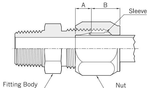
Fig-2 Assembly
