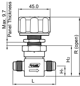
Male ZCR Fitting
