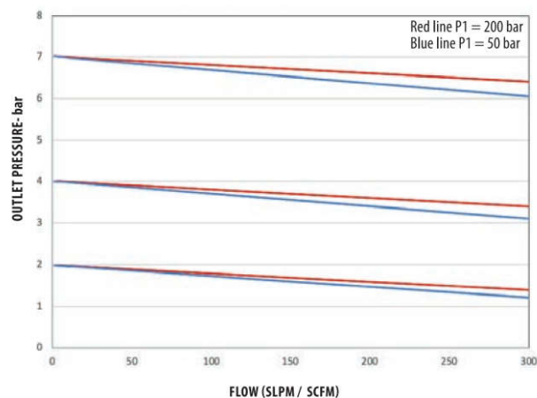
FLOW CURVES RX2400 HF (NITROGEN)
