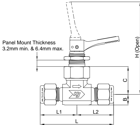
[ Straight pattern ]
