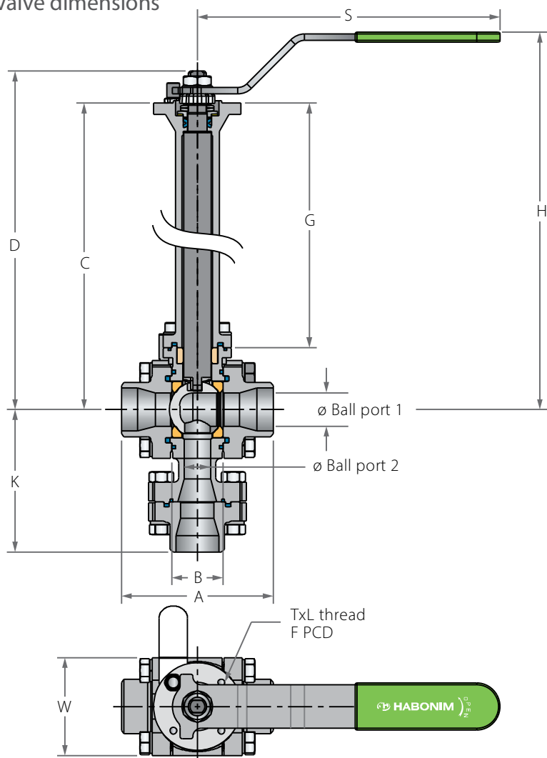
Valve dimensions
