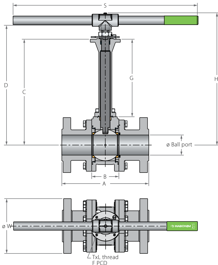
Valve dimensions
