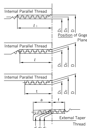
Fit of External Taper Thread to Internal Taper Thread or Internal Parallel Thread
