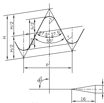
Basic profile of External Taper Thread and Internal Taper Thread
