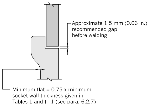
Fig. 2 Welding Gap and Minimum flat Dimensions for Socket - Welding Fittings
