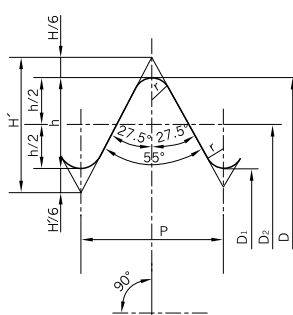
Basic profile of Internal Parallel Thread
